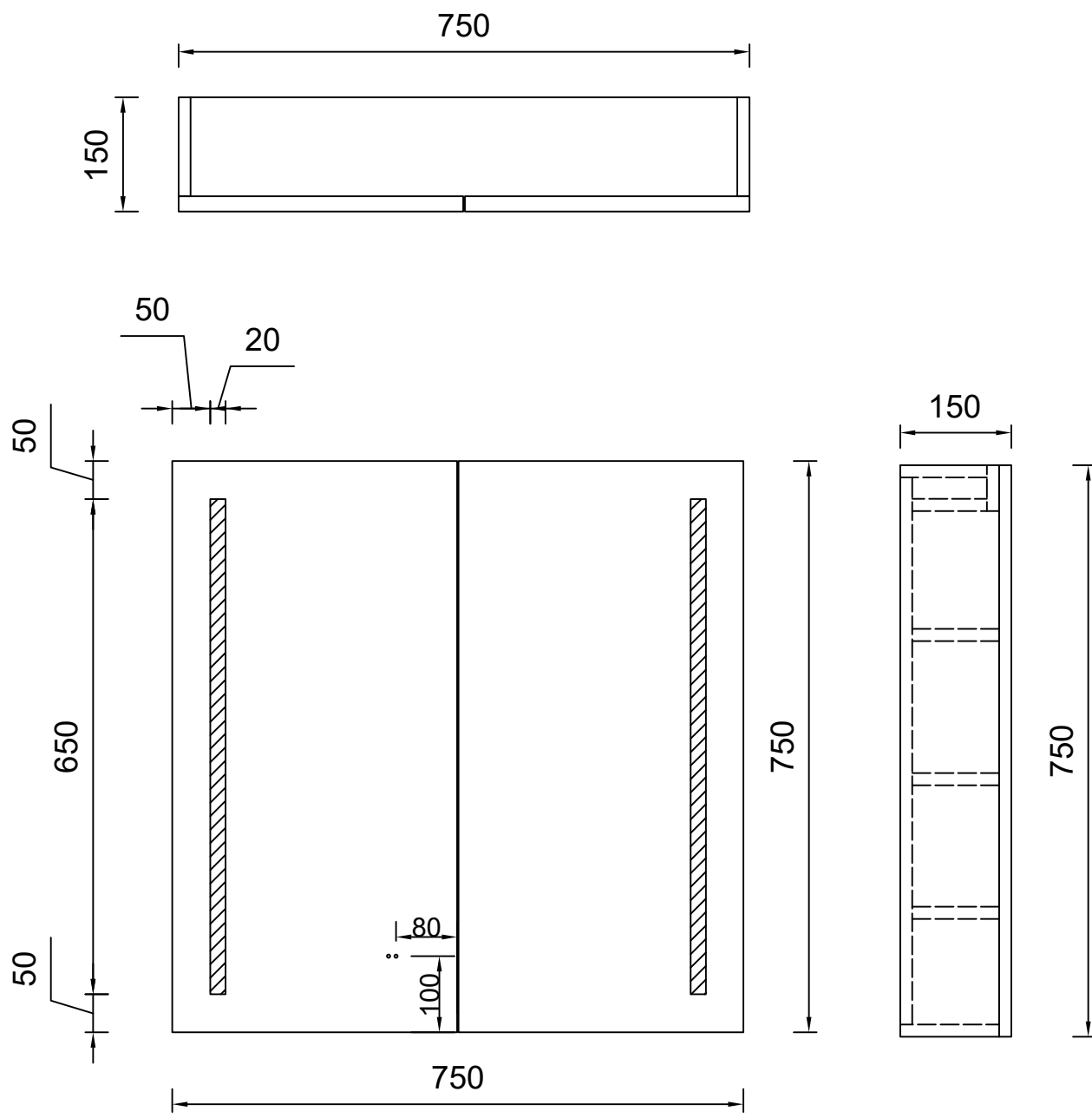
LED-PSH-7575
