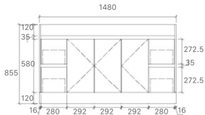
SY05-1500 Size: 1480x450x855mm
