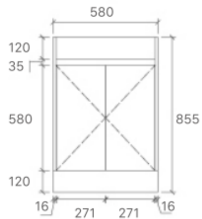
SY05-600 Size: 580x450x855mm
