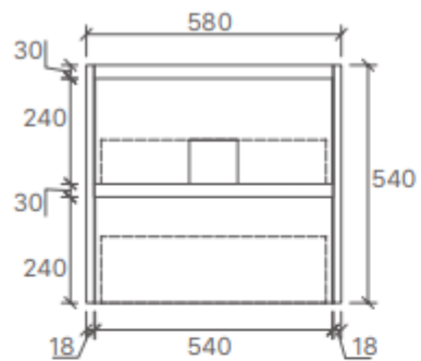
YOKO-600 Size: 580x455x540mm
