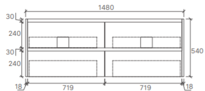
YOKO-1500D Size: 1480x455x540mm
