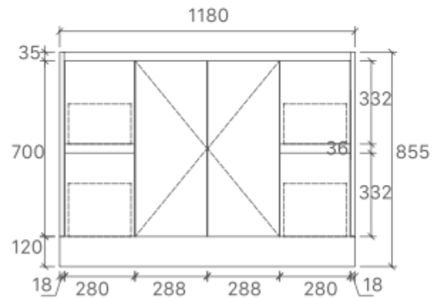
SK7-1200 Size: 1180x455x855mm
