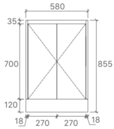
SK7-600 SIZE: 580x455x855mm
