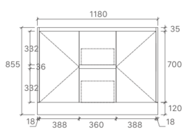
SK7-1200D Size: 1180x455x855mm
