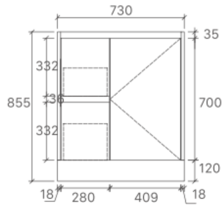
SK7-750L Size: 730x455x855mm
