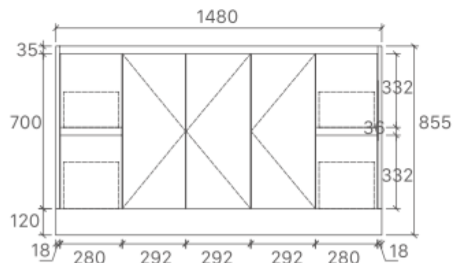
SK7-1500 Size: 1480x455x855mm
