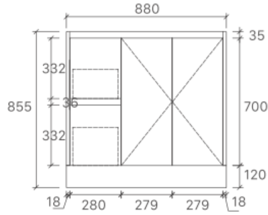
SK7-900L Size: 880x455x855mm
