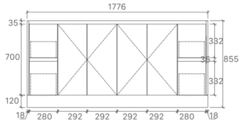
SK7-1800 Size: 1776x455x855mm
