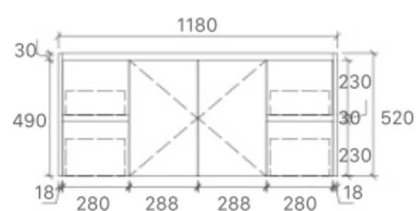
WH76-1200 Size: 1180x455x520mm
