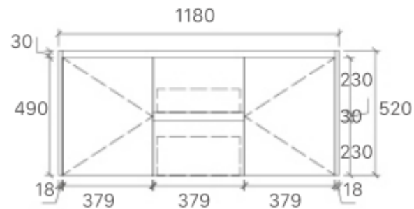
WH76-1200D Size: 1180x455x520mm
