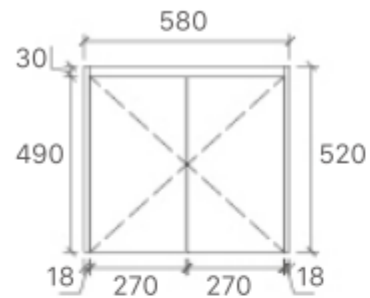
WH76-600 Size: 580x455x520mm
