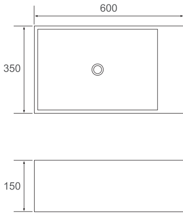
■ SAVANNAH SI-A12-600 Color: Matt White Size: 600x350x150mm
