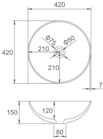
■ OTIS SI-A26G-420 or SI-A26-420 Color: Gloss White or Matt White Size: 420x420x150mm
