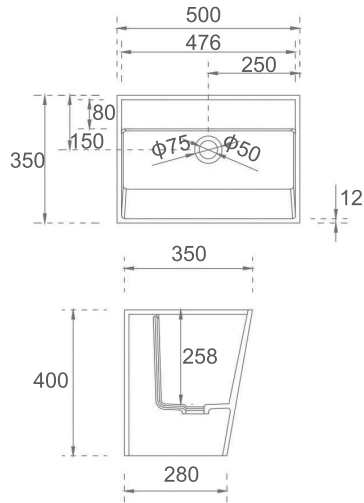
■ COMPACT SI-A18G-500 or SI-A18-500 Color: Gloss White or Matt White Size: 500x350x400mm
