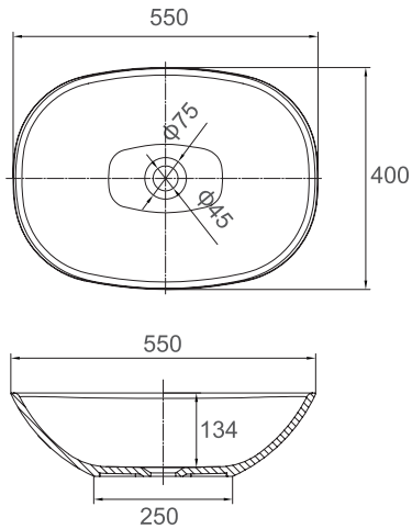
■ AMBER SI-M03G: Gloss White SI-M03: Matt White SI-M03B: Matt Black Size: 547x400x155mm
