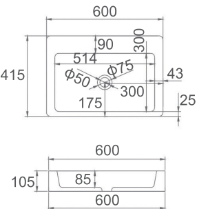
■ GRANDE-600 SI-A20G-600 or SI-A20-600 Color: Gloss White or Matt White Size: 600x415x105mm
