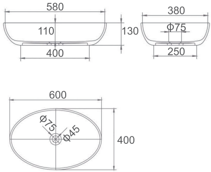
■ CECILY SI-A101G-600 or SI-A101-600 Color: Gloss White or Matt White Size: 600x400x130mm
