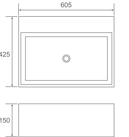
■ SPLIZE SI-A07G-605 or SI-A07-605 Color: Gloss White or Matt White Size: 605x425x150mm
