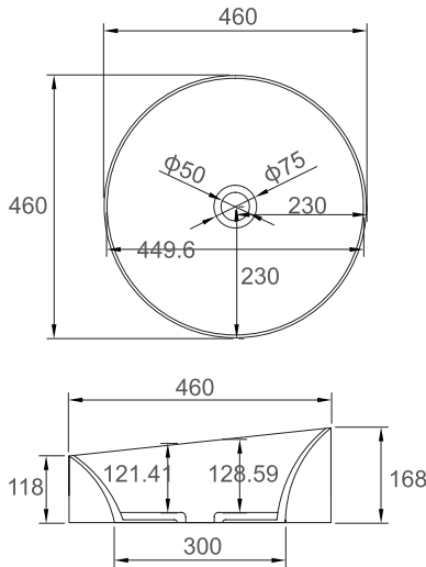
■ ODESSA SI-A19G-460 or SI-A19-460 Color: Gloss White or Matt White Size: 460x460x165mm
