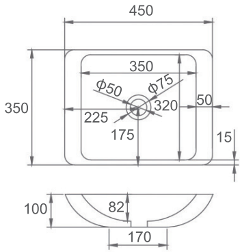
■ RIO-450 SI-A25G-450 or SI-A25-450 Color: Gloss White or Matt White Size: 450x350x100mm
