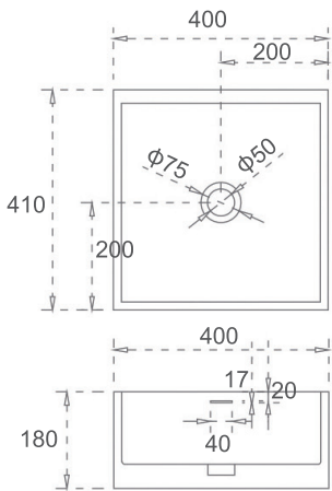
■ TITUS SI-A66G-410 or SI-A66-410 Color: Gloss White or Matt White Size: 410x400x180mm
