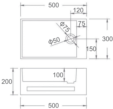
■ ZAYA SI-A17-500 (Wall Hung Basin) Color: Gloss White or Matt White Size: 500x300x200mm
