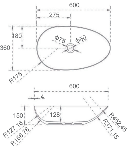
■ ABEL SI-A75G-600 or SI-A75-600 Color: Gloss White or Matt White Size: 600x350x160mm
