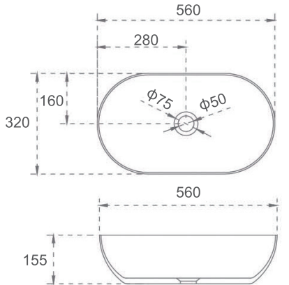
■ CHLOE SI-A78G-560 or SI-A78-560 Color: Gloss White or Matt White Size: 560x320x155mm
