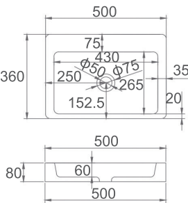
■ GRANDE-500 SI-A20G-500 or SI-A20-500 Color: Gloss White or Matt White Size: 500x500x80mm
