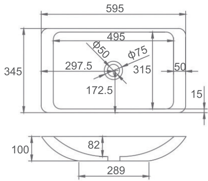
■ MONARCO SI-A22G-595 or SI-A22-595 Color: Gloss White or Matt White Size: 595x345x100mm
