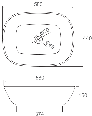
■ SELENE SI-M08G: Gloss White SI-M08: Matt White SI-M08B: Matt Black Size: 578x444x150mm
