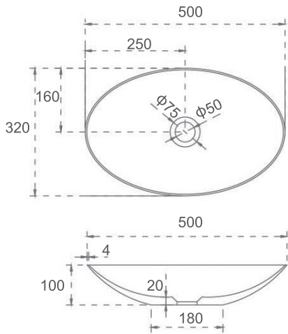
■ LYDIA SI-A73G-500 or SI-A73-500 Color: Gloss White or Matt White Size: 500x320x100mm
