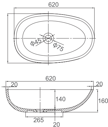
■ CRYSTAL SI-M02G: Gloss White SI-M02: Matt White SI-M02B: Matt Black Size: 611x358x158mm
