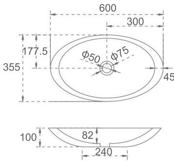
■ PHOENIX-600 SI-A23G-600 or SI-A23-600 Color: Gloss White or Matt White Size: 600x355x100mm
