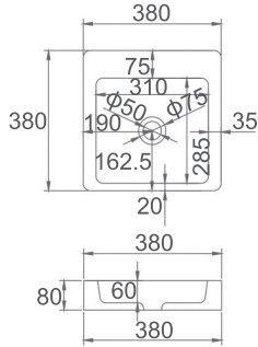
■ GRANDE-380 SI-A20G-380 or SI-A20-380 Color: Gloss White or Matt White Size: 380x380x80mm
