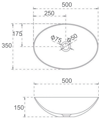
■ AMOS SI-A72G-500 or SI-A72-500 Color: Gloss White or Matt White Size: 500x350x150mm
