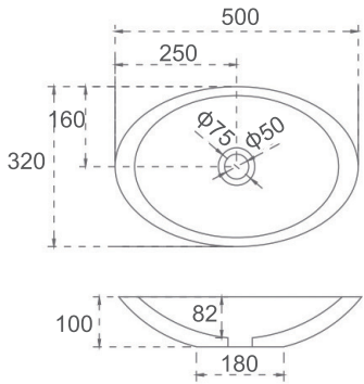
■ PHOENIX-500 SI-A23G-500 or SI-A23-500 Color: Gloss White or Matt White Size: 500x320x100mm
