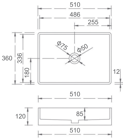
■ QUATTRO SI-A28G-510 or SI-A28-510 Color: Gloss White or Matt White Size: 510x360x115mm
