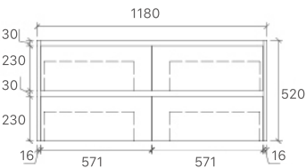
SYWH04-1200S Size: 1180x455x520mm
