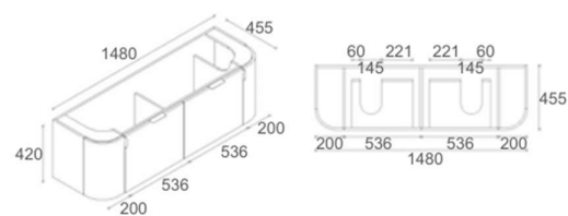
CWH66-1500D Size: 1480x455x420mm
