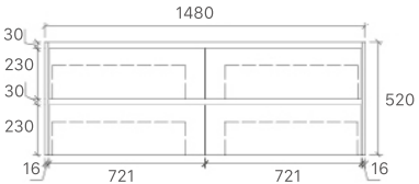
SYWH04-1500S Size: 1480x455x520mm
