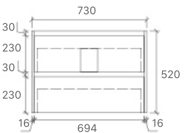
SYWH04-750 Size: 730x455x520mm
