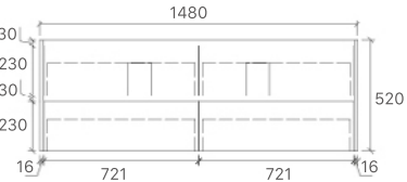
SYWH04-1500D Size: 1480x455x520mm
