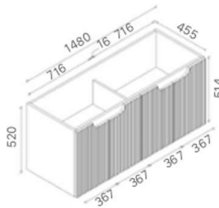
WH56-1500D Size: 1480x455x520mm
