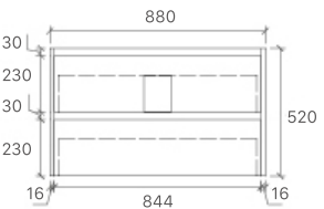
SYWH04-900 Size: 880x455x520mm
