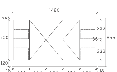
SK7-1500 Size: 1480x455x855mm
