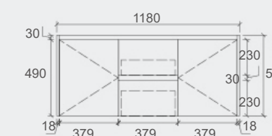
WH76-1200D Size: 1180x455x520mm
