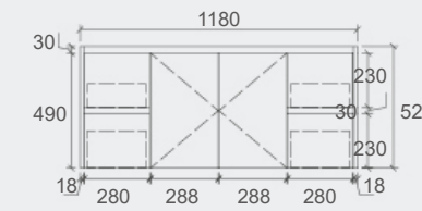
WH76-1200 Size: 1180x455x520mm
