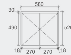
WH76-600 Size: 580x455x520mm
