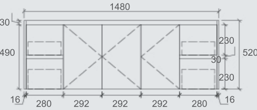
SYWH05-1500 Size: 1480x455x520mm
