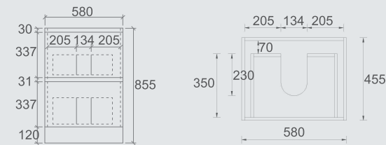
CORE-600 Size: 580x455x855mm
