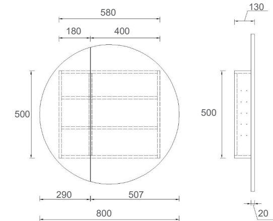
RSC-800 Φ800x800x130mm
