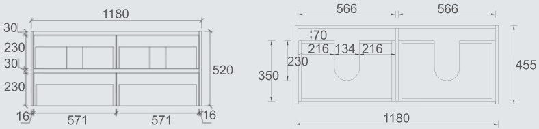
SYWH04-1200D Size: 1180x455x520mm
