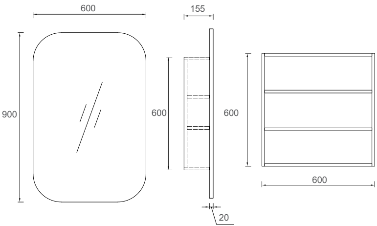
RSH-6090 600x900x155mm
