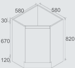
PC6060 Corner: 580x580x820mm
