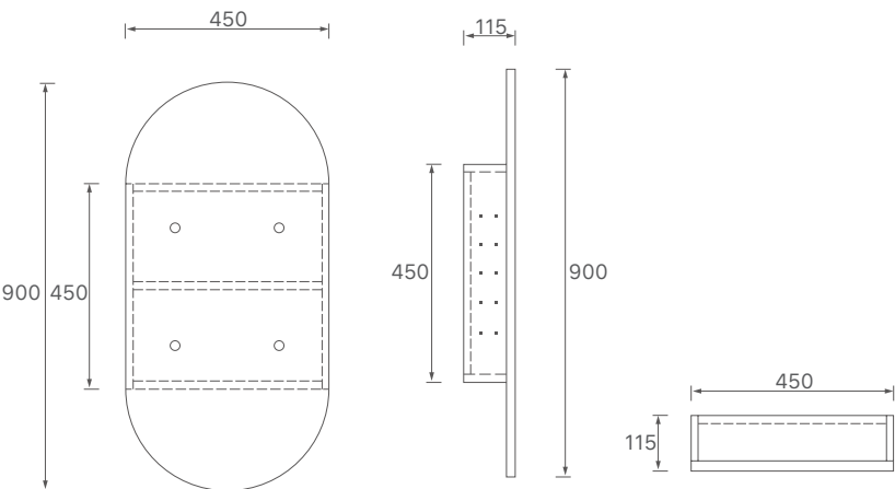
OSH-4590 450x900x115mm
