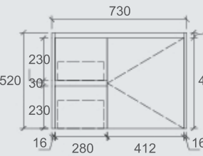
SYWH05-750L Size: 730x455x520mm
