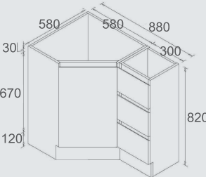
PC6090 Coner: 580x880x820mm
