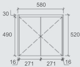
SYWH05-600 Size: 580x455x520mm
