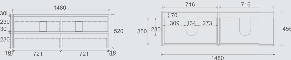
SYWH04-1500D Size: 1480x455x520mm
