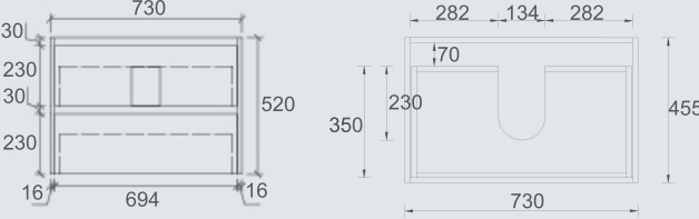
SYWH04-750 Size: 730x455x520mm
