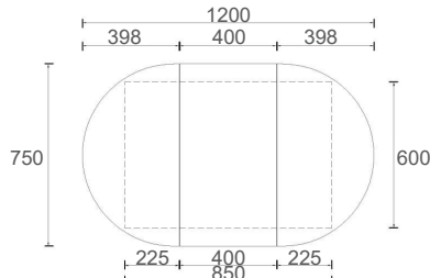
OSH-12075 1200x750x146mm
