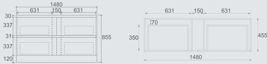
CORE-1500 Size: 1480x455x855mm
