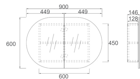
OSH-9060 900x600x146mm
