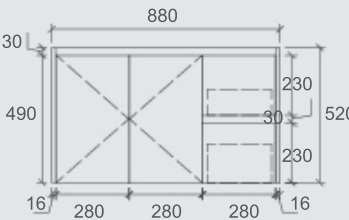
SYWH05-900R Size: 880x455x520mm
