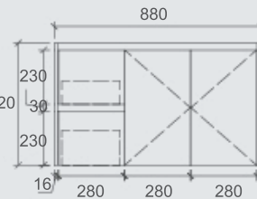
SYWH05-900L Size: 880x455x520mm
