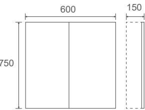
PSH-6075 600x750x150mm
