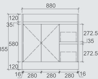
SY05-900R Size: 880x455x855mm
