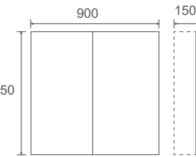
PSH-9075 900x750x150mm
