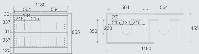
CORE-1200D Size: 1180x455x855mm
