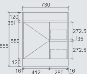
SY05-750R Size: 730x455x855mm
