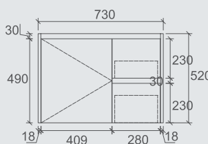
WH32-750R Size: 730x355x520mm
