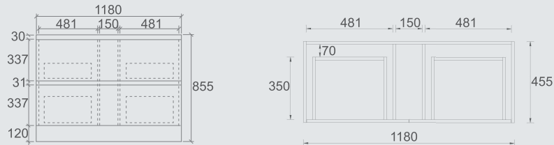
CORE-1200 Size: 1180x455x855mm
