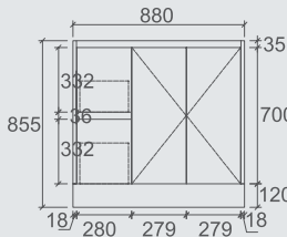
SK32-900L Size: 880x355x855mm
