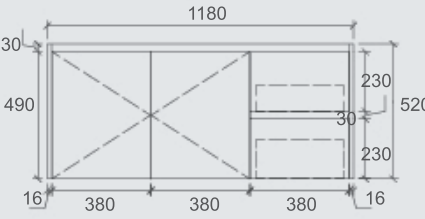
SYWH05-1200R Size: 1180x455x520mm
