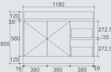
SY05-1200R Size: 1180x455x855mm
