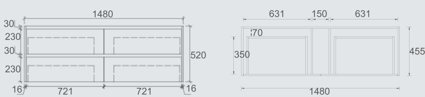
SYWH04-1500 Size: 1480x455x520mm
