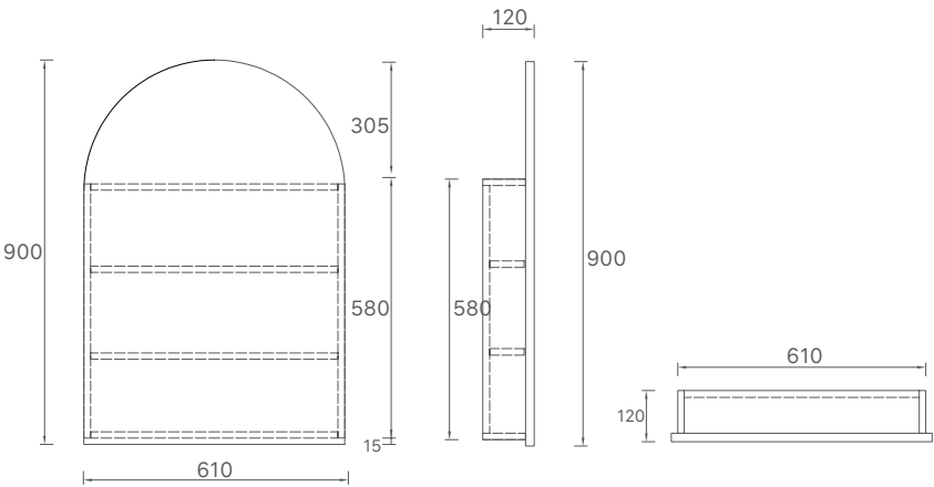
ASH-6161 610x900x120mm
