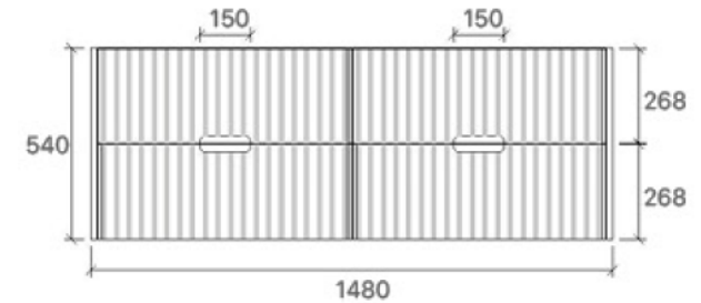
WH86-1500D Size: 1480x455x540mm
