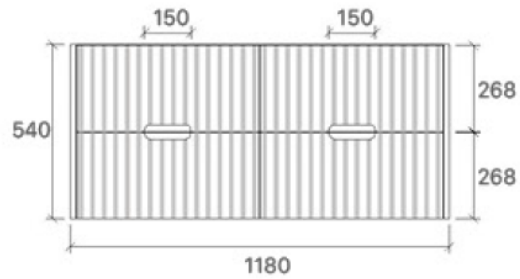
WH86-1200 Size: 1180x455x540mm
