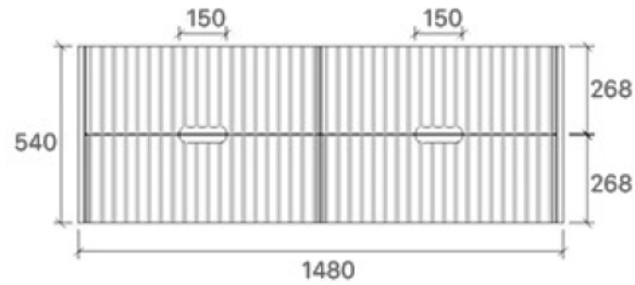
WH86-1500 Size: 1480x455x540mm
